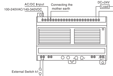
(Fig.3.2 Remote Control application)
