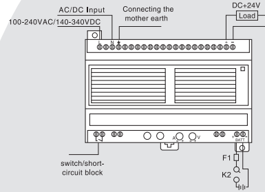
(Attn: the connection of the positive and negative pole) (Fig.3.3 UPS application)
